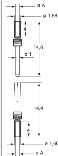
CIF and CIM contacts
