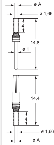
RIF and RIM contacts
