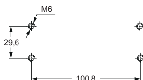
panel cut-out for MGK 2AP25
