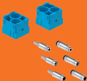
MIXO pneumatic metal modules and contacts
