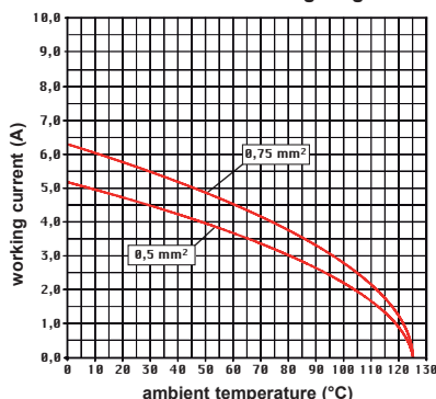
CX IBF/IBM 25 poles connector inserts Maximum current load derating diagram
