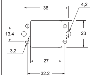
panel cut-out for CQ IA - CQ IAP enclosure
