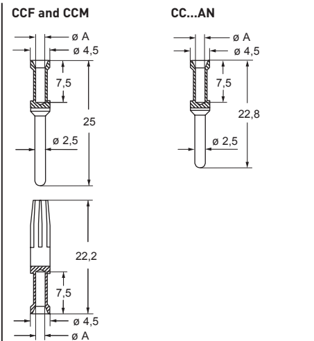
CCF, CCM and CC..AN contacts
