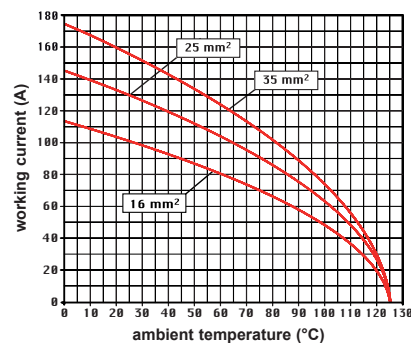
CX 02 poles connector inserts Maximum current load derating diagram
