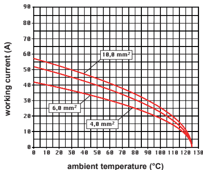
CQ 12 poles connector inserts Maximum current load derating diagram
