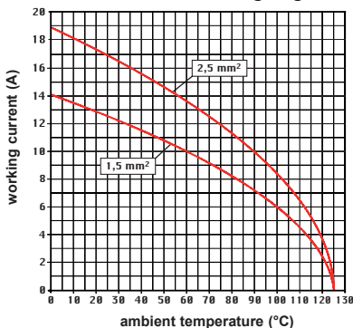
CX 05 SHF/SHM power poles connector inserts Maximum current load derating diagram
