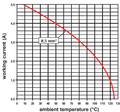
CX IF/IM 25 poles connector inserts Maximum current load derating diagram
