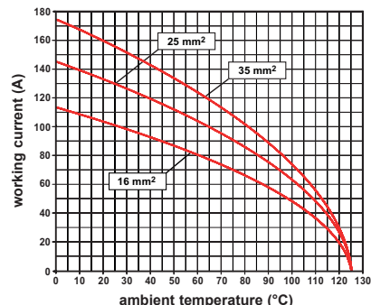
CX 01 poles connector inserts Maximum current load derating diagram
