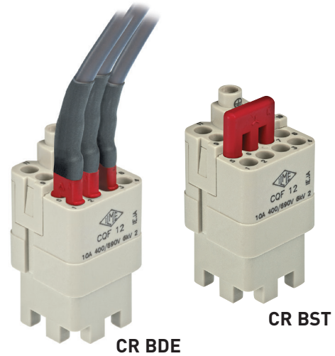
Bridges for delta or star connection from page 694, 695
