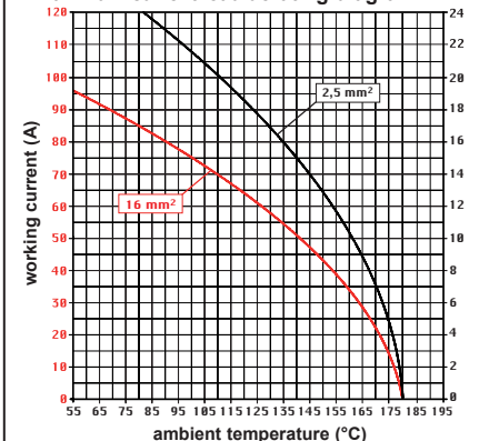
CX RY 4/8 poles connector inserts Maximum current load derating diagram
