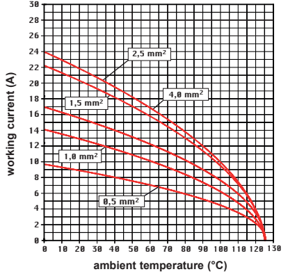
CDC 16 poles connector inserts Maximum current load derating diagram
