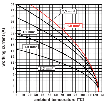
CMCE 12 poles connector inserts Maximum current load derating diagram
