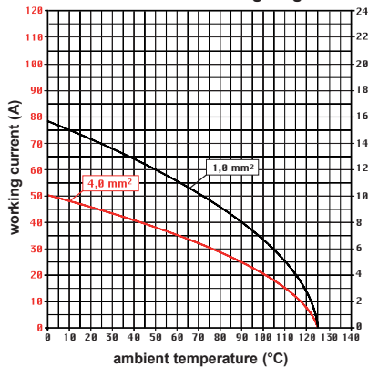
CX 4/8 poles connector inserts Maximum current load derating diagram
