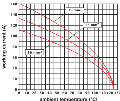
CGX 6/6 power poles connector inserts Maximum current load derating diagram
