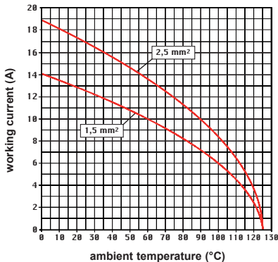
CX 05 poles connector inserts Maximum current load derating diagram
