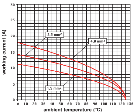
RQEE 64 poles connector inserts Maximum current load derating diagram
