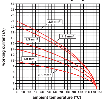
CDA 3 poles connector inserts Maximum current load derating diagram
